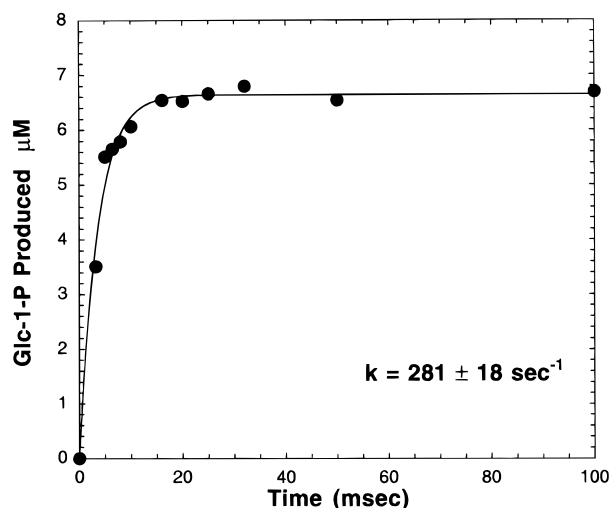
FIGURE 3: Time course for wild-type enzyme uridylylation observed by transient phase kinetics. 129 \mu\text{M} wild-type and 10.2 mM UDP-glucose were reacted at 4 ^{\circ}\text{C} and quenched at given times using 0.5 M HCl. The amount of Glc-1-P produced at each time point is plotted as a function of time. The time points were fitted to a first-order rate equation which gave a first-order rate constant of 281 \pm 18 \text{ s}^{-1} . The overall turnover number for the enzyme at 4 ^{\circ}\text{C} is 62 \pm 8 \text{ s}^{-1} . This indicates that uridylylation of wild-type uridylyltransferase is kinetically competent.
