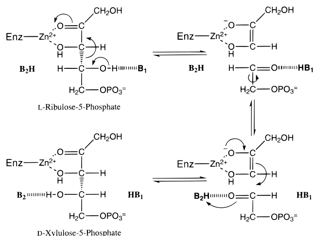
FIGURE 10: Proposed mechanism of the L-Ru5P 4-epimerase-catalyzed reaction. The diagram depicts an aldol cleavage–condensation mechanism for conversion of L-Ru5P to D-Xu5P that involves substrate to metal binding and a cis enediolate-stabilized intermediate.
